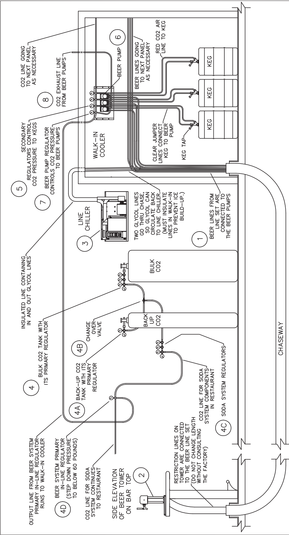
BEER PUMP INSTALLATION DRAWING FOR BULK CO2 WITH BACK-UP TANK PRIMARY REGULATOR EXPLANATION: 4 – Main Bulk CO2 regulator output to changeover valve 4A – Back-up CO2 regulator output to changeover 4B – Changeover valve output goes to soda system regulators 4C – Main soda system regulator bank output goes to components in restaurant 4D – Primary in-line regulator for beer system T's into soda system line as it travels to restaurant with output for beer to walk-in cooler
